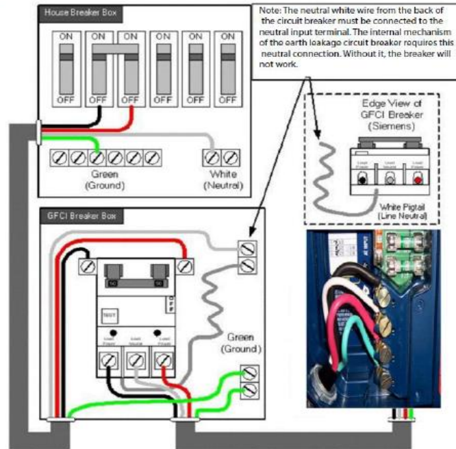
Figure 3 - Cable schematics Consult the caliber chart page 11
