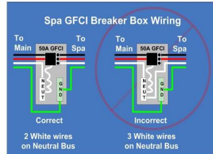
Figure 2 - GFCI Wiring
